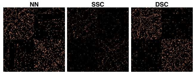
Fig. 1. Subset selection from overlapping subspaces in noise (60% overlap, SNR = 20dB); from left to right: NN, SSC, and the proposed DSC.
