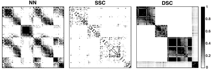
Fig. 3. Affinity matrices from face illumination subspaces; from left to right: NN, SSC, and DSC.
