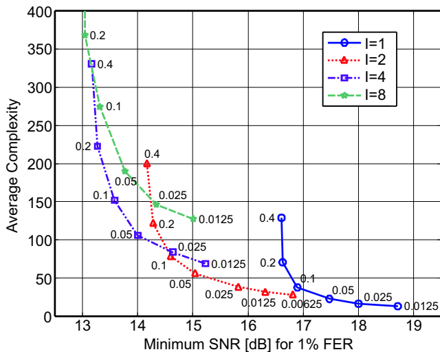
Fig. 2. Performance/complexity trade-off of the SISO STS-SD with sorted QR decomposition (SQRD) as described in [13]. The numbers next to the curves correspond to normalized LLR clipping levels and I denotes the number of iterations over the MIMO detector (and the channel decoder).
