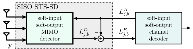
Fig. 1. Iterative MIMO decoder [4]. The SISO STS-SD (corresponding to the dashed box) directly computes extrinsic log-likelihood ratios.
